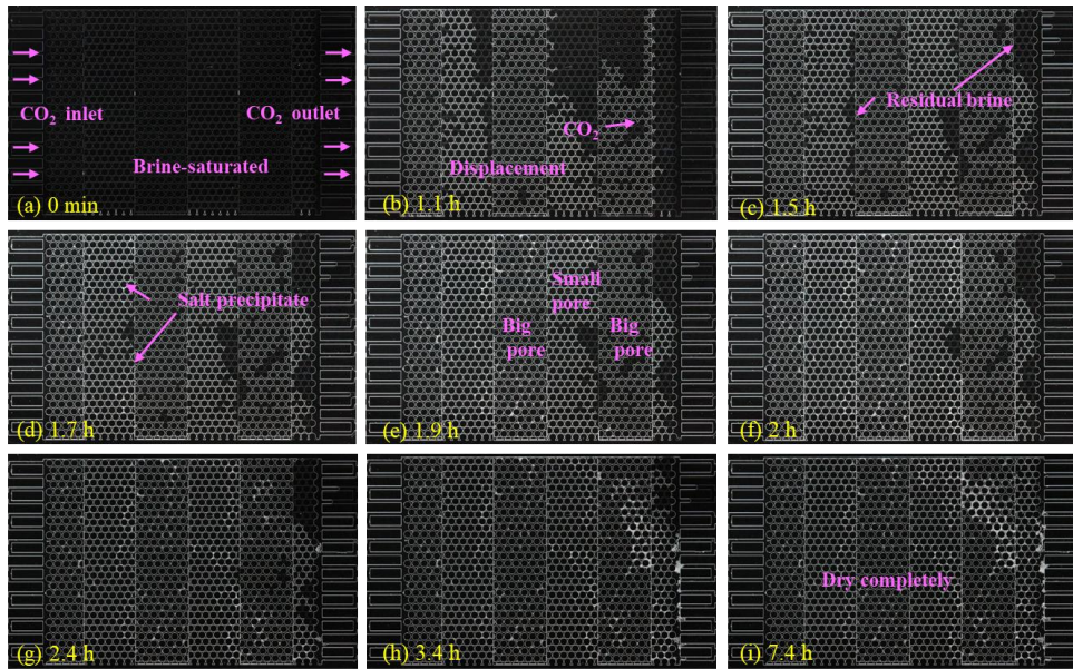
Fig.S3 Salt precipitation process of case LR-2
