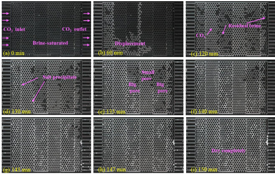
Fig.S4 Salt precipitation process of case LR-3
