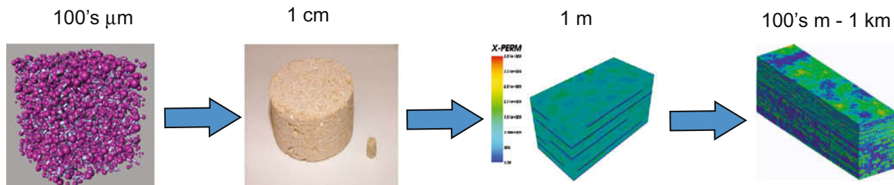
Fig. 14. A schematic of a potential upscaling method for flow and transport in porous media, integrating simulation approaches and data at different scales (Rhodes, 2008).
