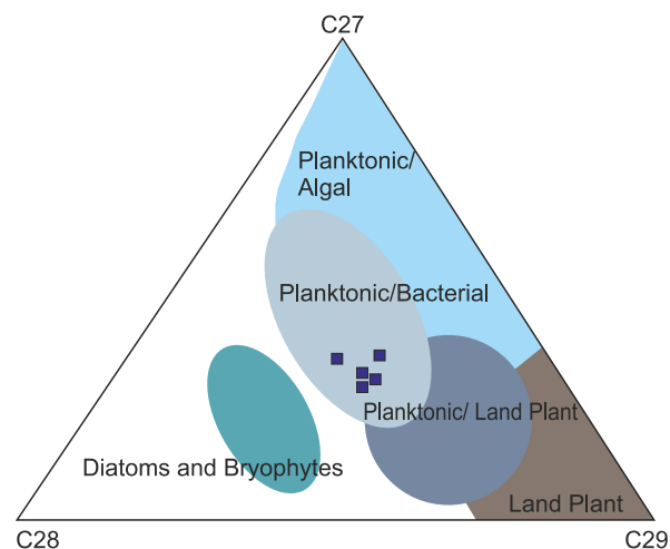
Fig. 3. Sterane ternary diagram of C 27 %, C 28 % and C 29 % (αααR) concerning the selected samples in Bozbel and Kozluca Formations.
