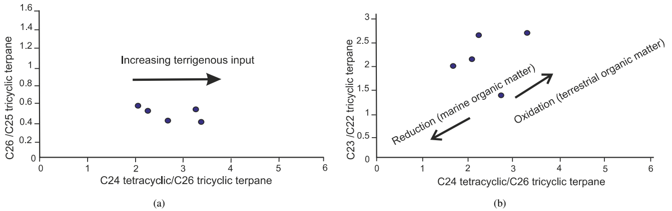
Fig. 4. a) Relationships between C 26 /C 25 tricyclic terpane vs C 24 tetracyclic/C 26 tricyclic terpane ratios, b) C 23 /C 22 tricyclic terpane vs C 24 tetracyclic/C 26 tricyclic terpane ratios for Eocene sediments.
