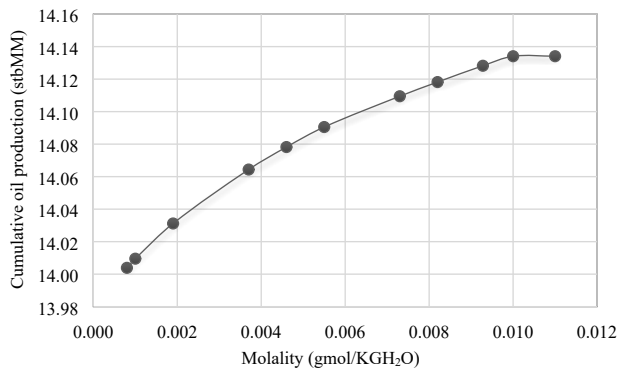
Fig. 10. Effect of Ca 2+ concentration in LSWF.
