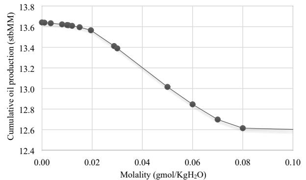
Fig. 12. Effect of Na + concentration in LSWF.
