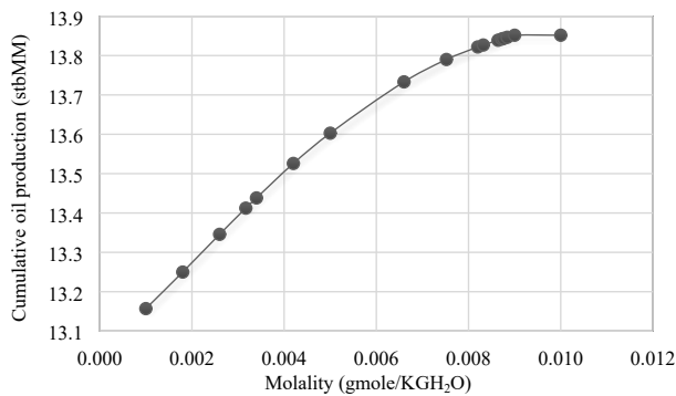
Fig. 11. Effect of Mg 2+ concentration in LSWF.
