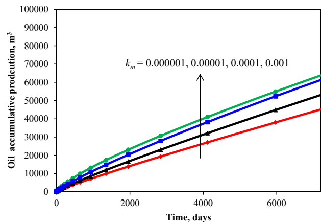
Fig. 9. Oil accumulative production in 20 years predicted with different matrix permeability.
