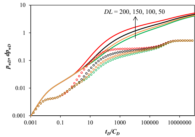
Fig. 12. Effect of fracture spacing on transient pressure curves.
