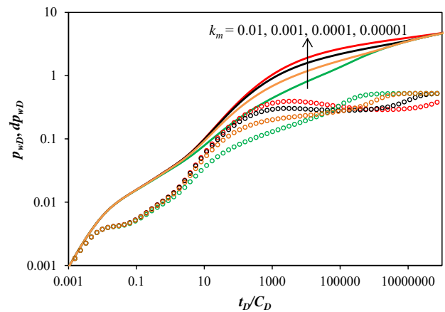
Fig. 8. Effect of matrix permeability on transient pressure curves.
