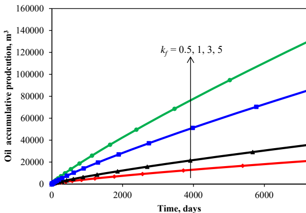
Fig. 7. Oil accumulative production in 20 years predicted with different natural fracture permeability.
