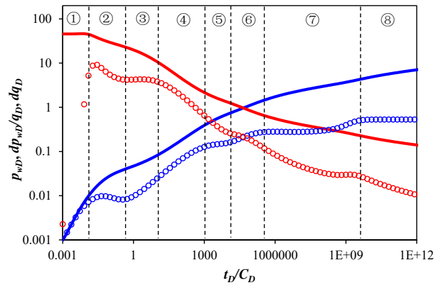
Fig. 4. Type curves for MsFHW. Basic parameters: M = 3 ; DL_D = 10 ; L_f = 50 ; \omega = 0.015 ; \lambda = 0.00001 ; C_D = 0.00001 ; S = 0.02 ; R_{fD} = 20 .
