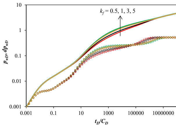
Fig. 6. Effect of natural fracture permeability on transient pressure curves.
