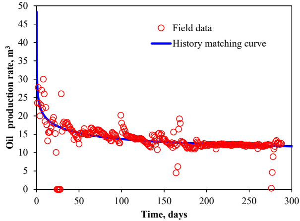
Fig. 5. History matching between the model result and real production data.
