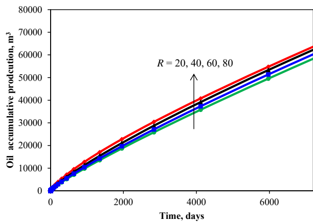
Fig. 11. Oil accumulative production in 20 years predicted with different matrix size.
