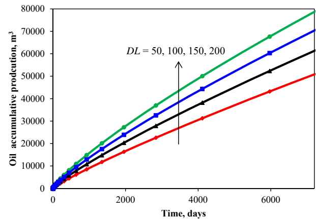
Fig. 13. Oil accumulative production in 20 years predicted with different fracture spacing.
