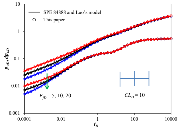
Fig. 3. Comparison of pressure and pressure derivative for multistage fractured horizontal well by 3 hydraulic fractures.
