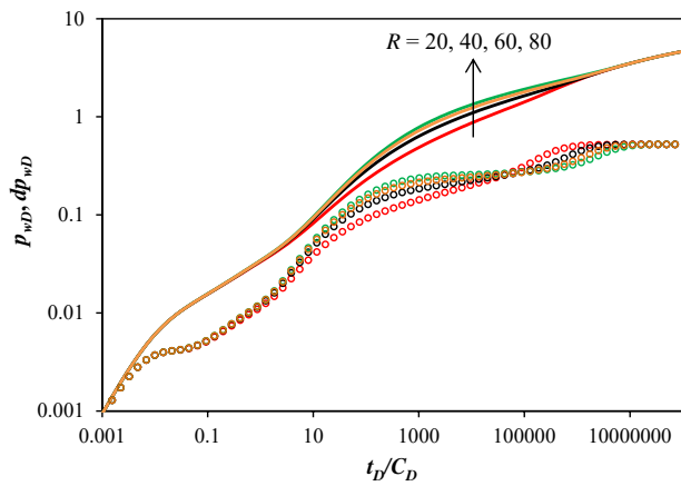
Fig. 10. Effect of matrix size on transient pressure curves.
