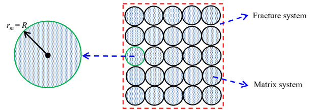
Fig. 2. Schematic of fracture and matrix system (after Yuan et al., 2018).
