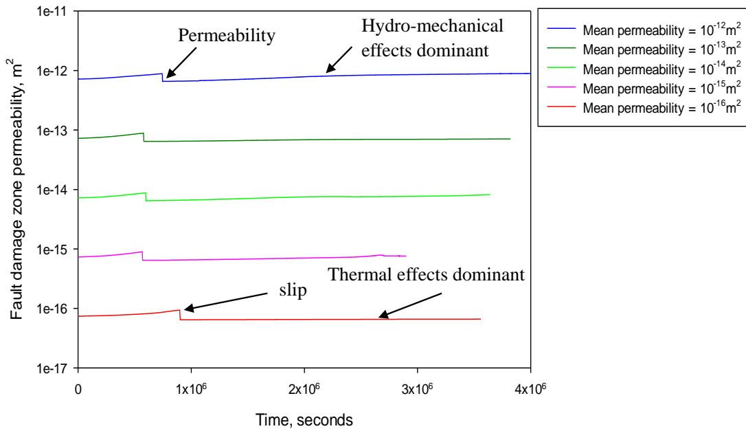
Fig. 4. Fracture permeability evolution for initial permeabilities ranging from 10^{-16} to 10^{-12} m^2 .
