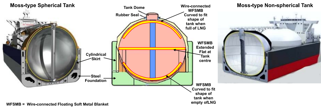
Fig. 15. MOSS-type rigid spherical and KHIs non-spherical shaped LNG tanks. Conceptual image of wire-connected blanket (WFSMB) in action in a MOSS-type tank. Left diagram (modified after: Mokhtab et al., 2014; Cult of Sea, 2017) and right diagram from (Kawasaki, 2017); Liquefied Gas Carriers , 2019
