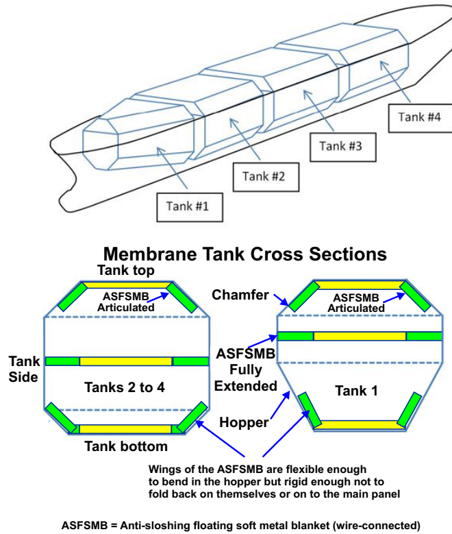
Fig. 13. The articulated ASFSMB involves three articulated components, a central, permanently flat section and two narrower wings that fold into the angles of the chamfer and hopper of membrane tanks as LNG fluid levels dictate.
